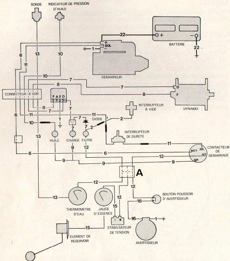
FIGURE 5/30. SCHEMA DE CABLAGE
